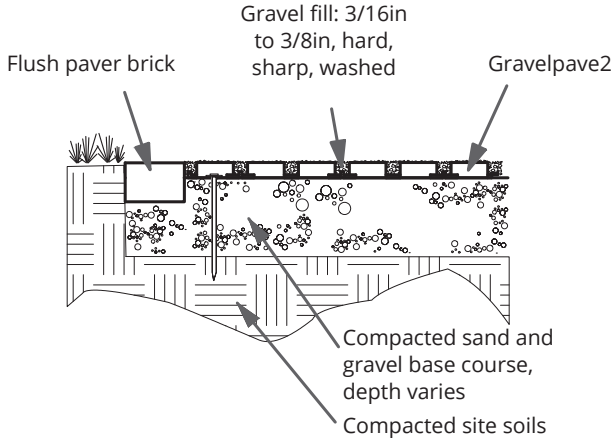
FLUSH BRICK PAVER EDGING
