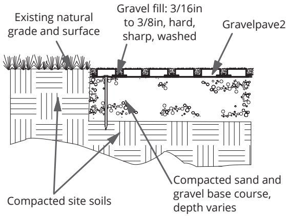
FLUSH, NATURAL (EXISTING) EDGING
