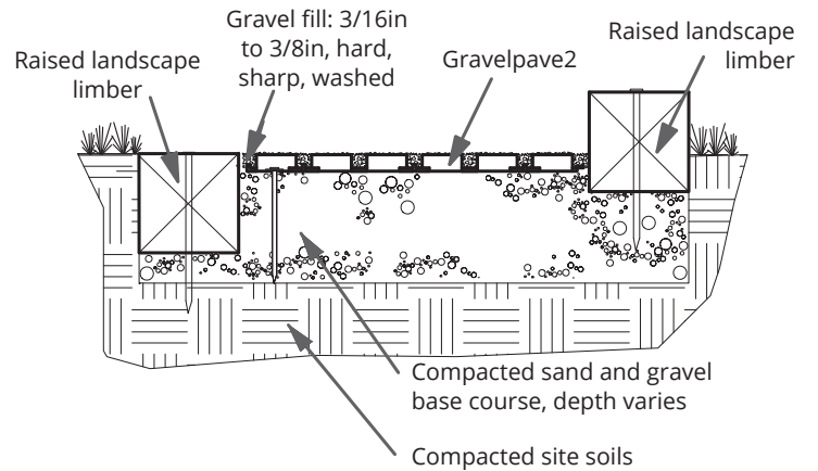
LANDSCAPE TIMBER EDGING
